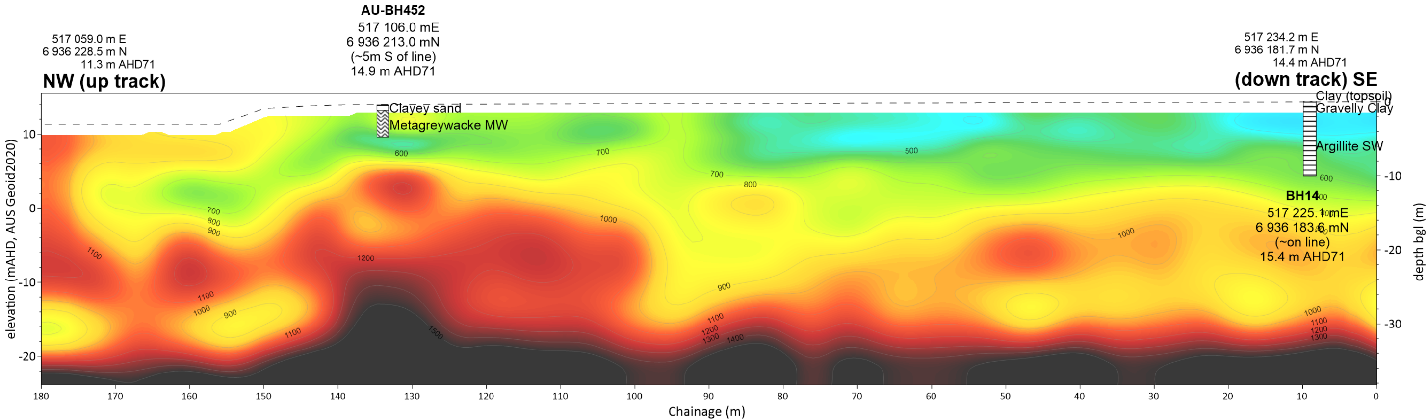
Seismic Line MASW AU-GP 172
